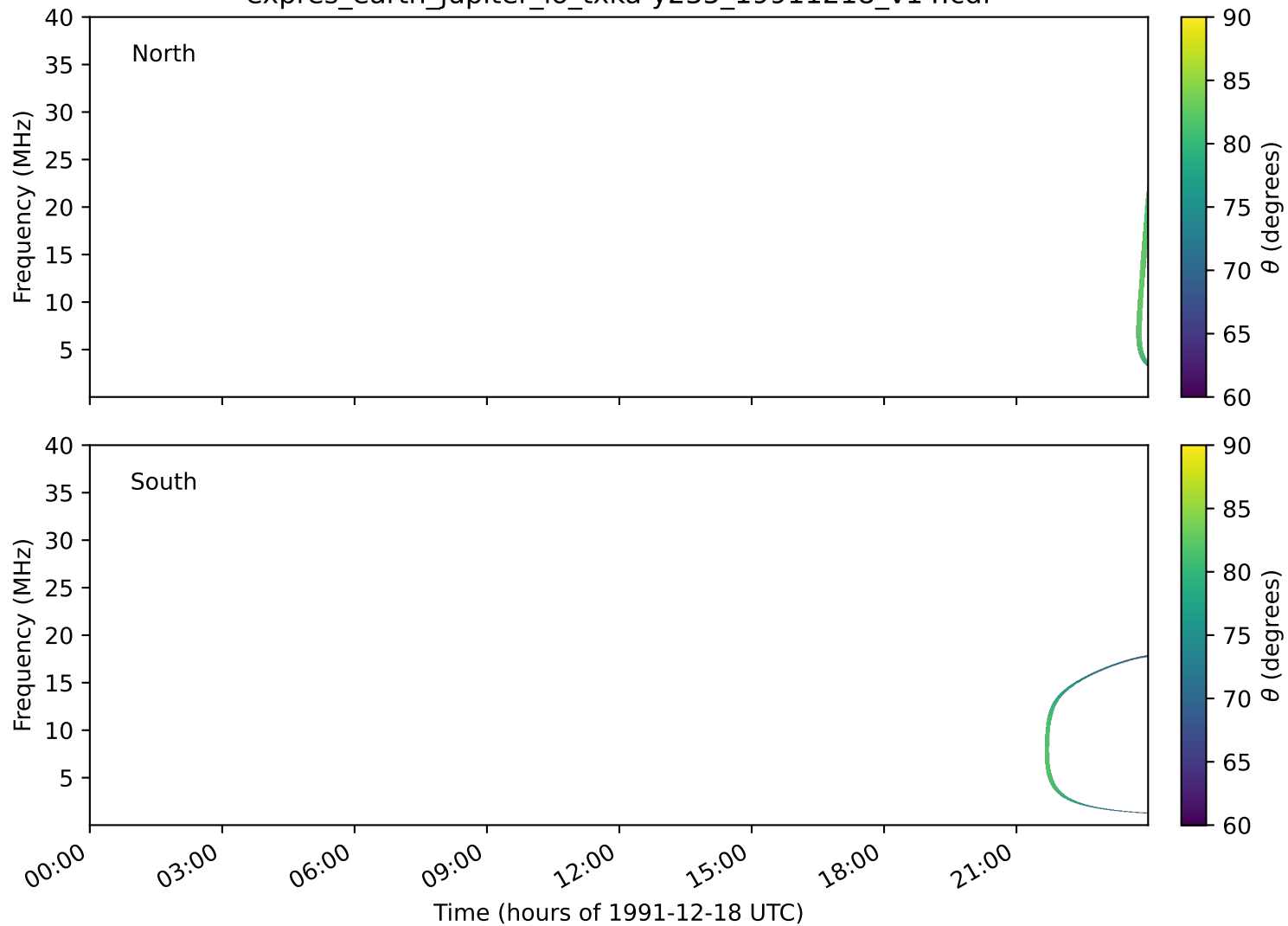
expres_earth_jupiter_io_txka-y235_19911218_v14.cdf
