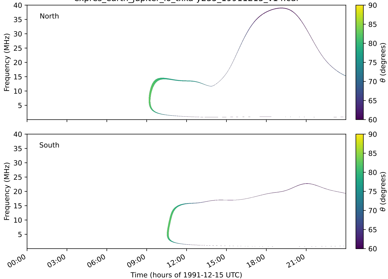
expres_earth_jupiter_io_txka-y235_19911215_v14.cdf
