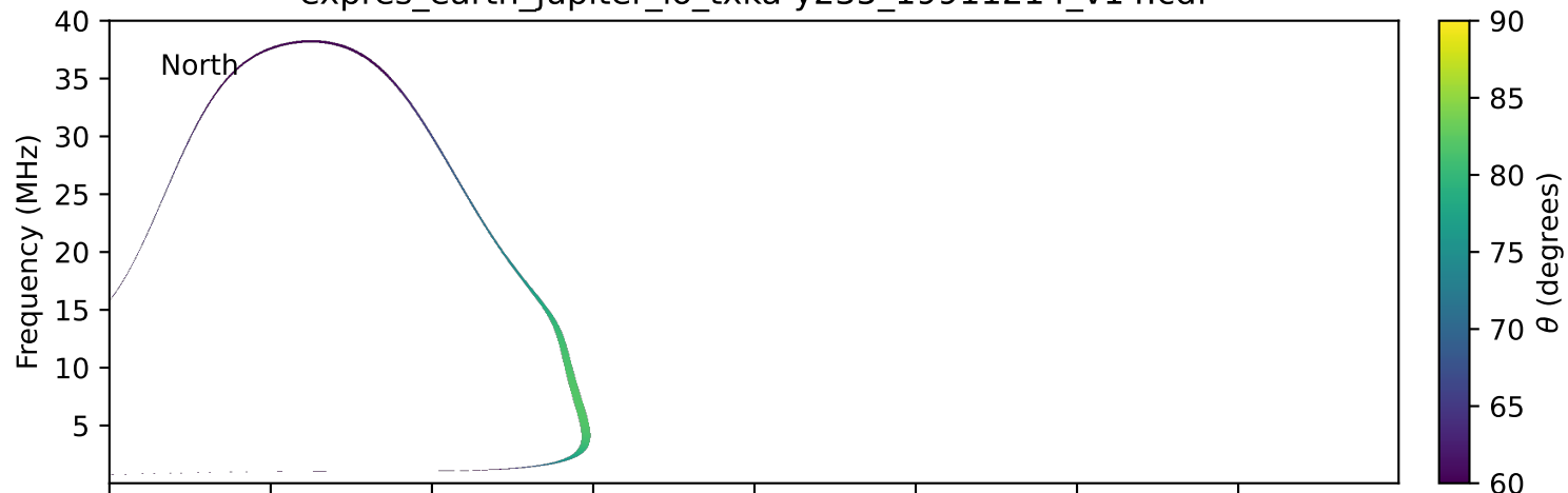
expres_earth_jupiter_io_txka-y235_19911214_v14.cdf
