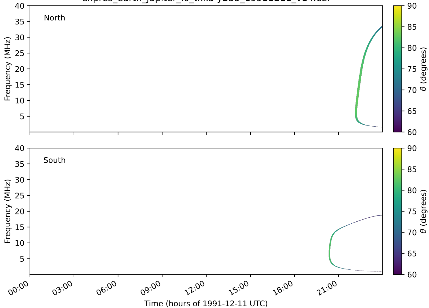
expres_earth_jupiter_io_txka-y235_19911211_v14.cdf
