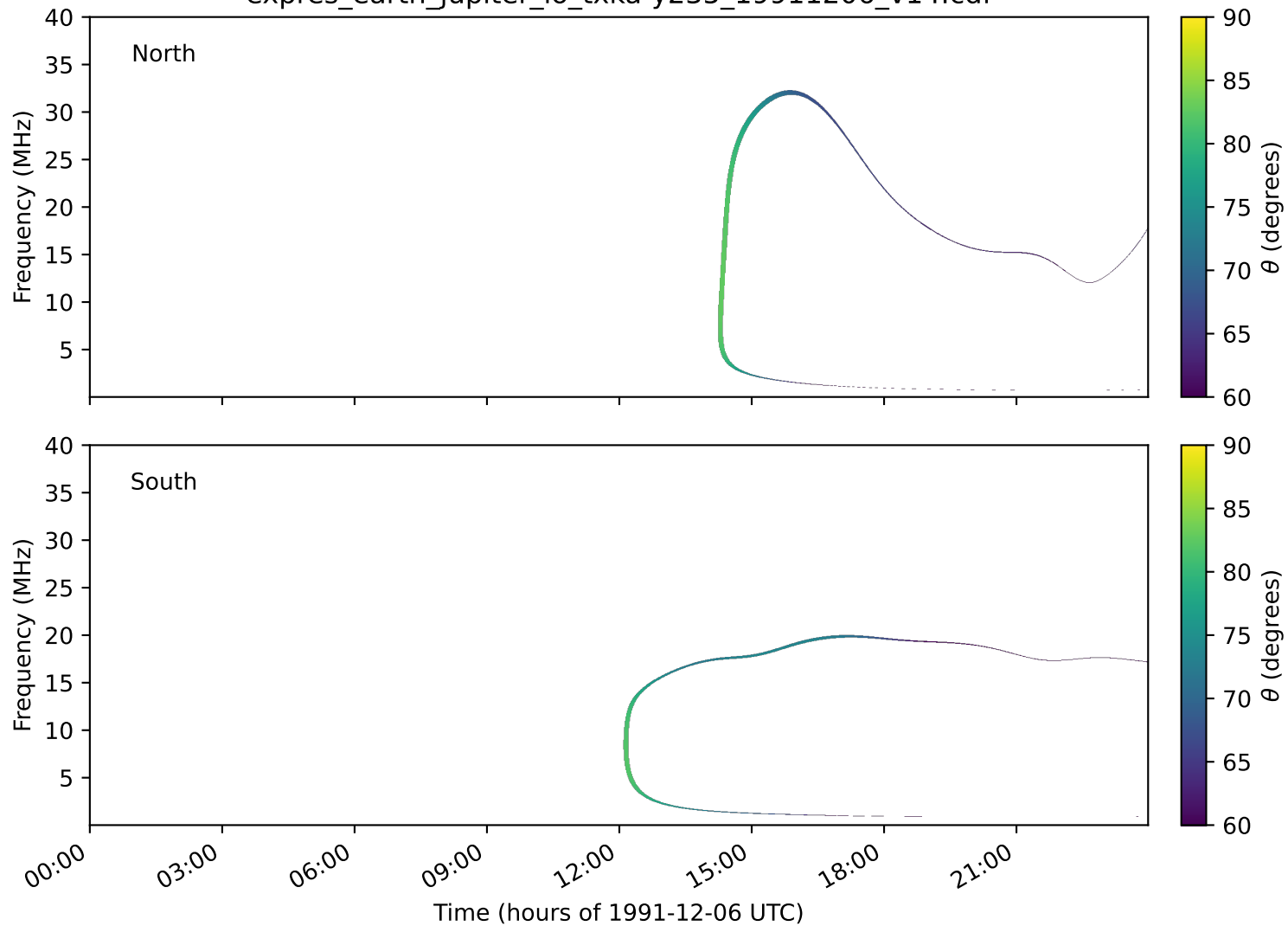
expres_earth_jupiter_io_txka-y235_19911206_v14.cdf
