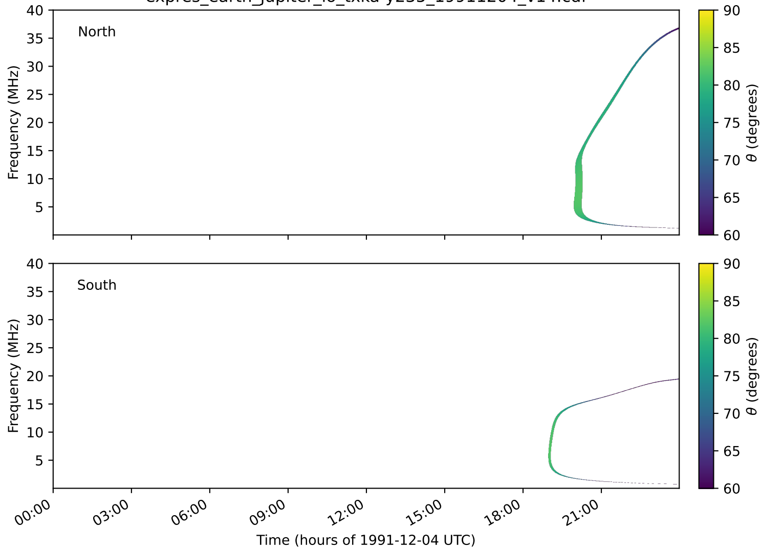
expres_earth_jupiter_io_txka-y235_19911204_v14.cdf
