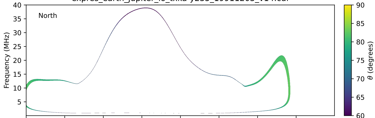
expres_earth_jupiter_io_txka-y235_19911203_v14.cdf
