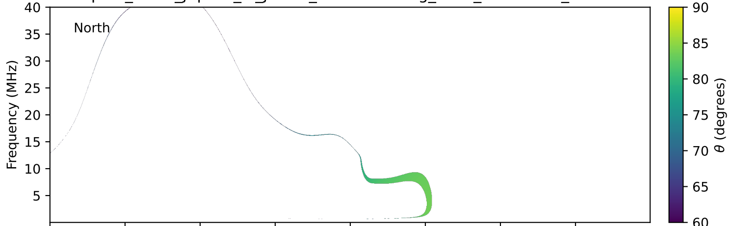
expres_earth_jupiter_io_jrm33_lossc-wid1deg_3kev_19911228_v11.cdf
