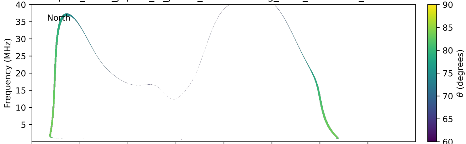
expres_earth_jupiter_io_jrm33_lossc-wid1deg_3kev_19911226_v11.cdf
