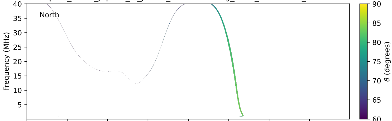
expres_earth_jupiter_io_jrm33_lossc-wid1deg_3kev_19911212_v11.cdf
