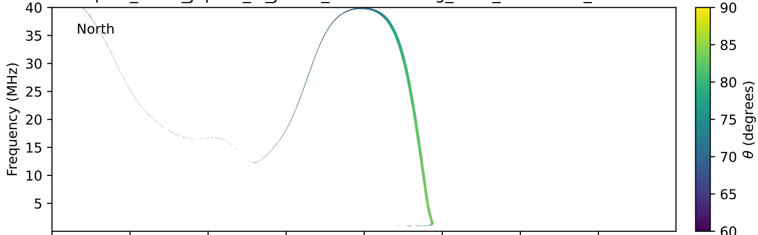
expres_earth_jupiter_io_jrm33_lossc-wid1deg_3kev_19911205_v11.cdf
