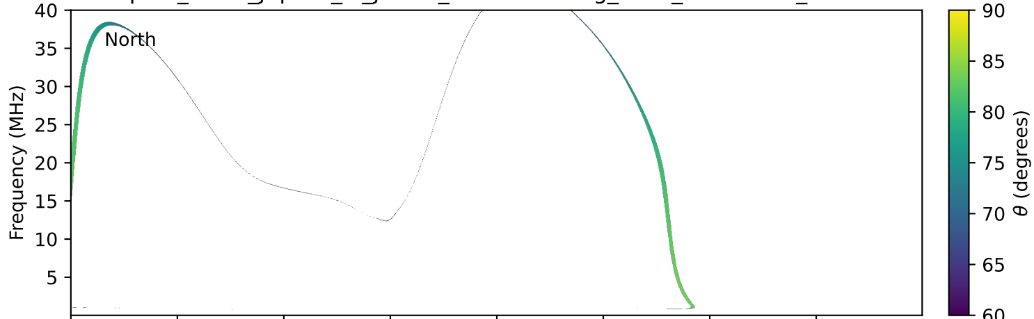
expres_earth_jupiter_io_jrm09_lossc-wid1deg_3kev_19911219_v11.cdf
