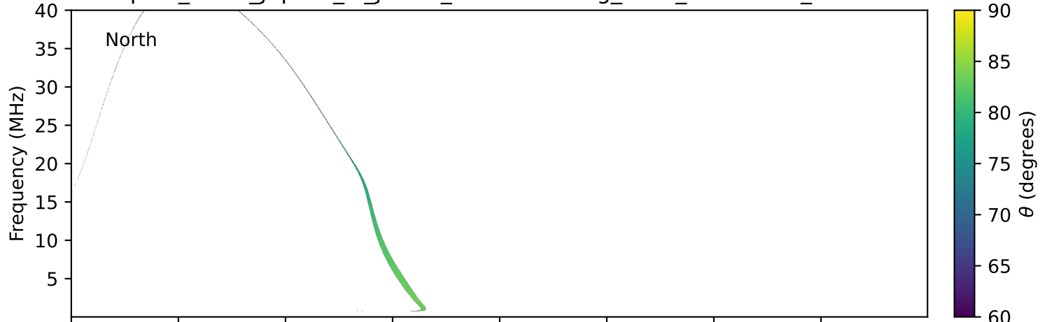
expres_earth_jupiter_io_jrm09_lossc-wid1deg_3kev_19911214_v11.cdf
