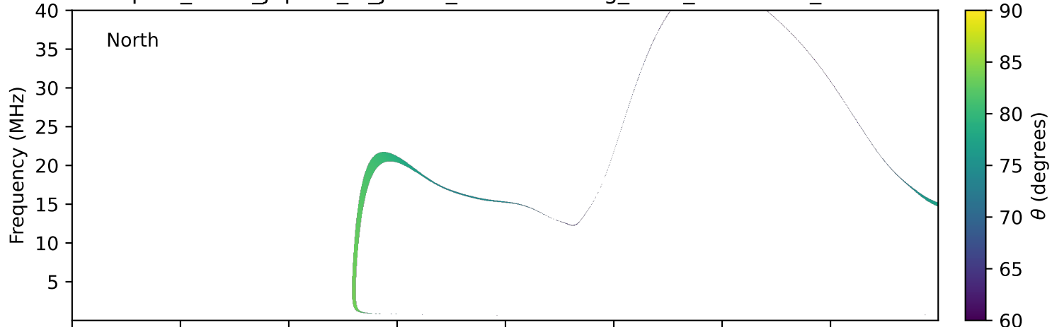
expres_earth_jupiter_io_jrm09_lossc-wid1deg_3kev_19911208_v11.cdf
