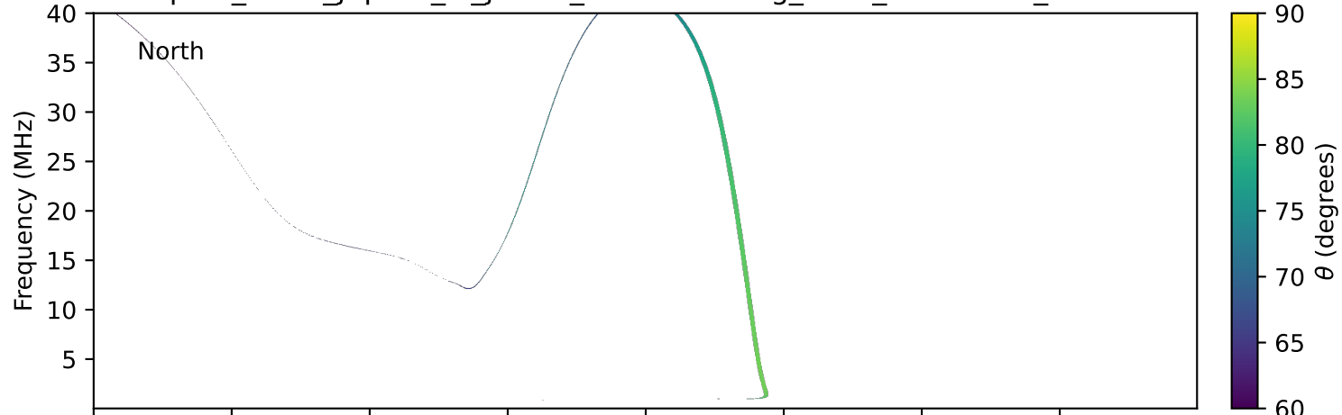
expres_earth_jupiter_io_jrm09_lossc-wid1deg_3kev_19911205_v11.cdf
