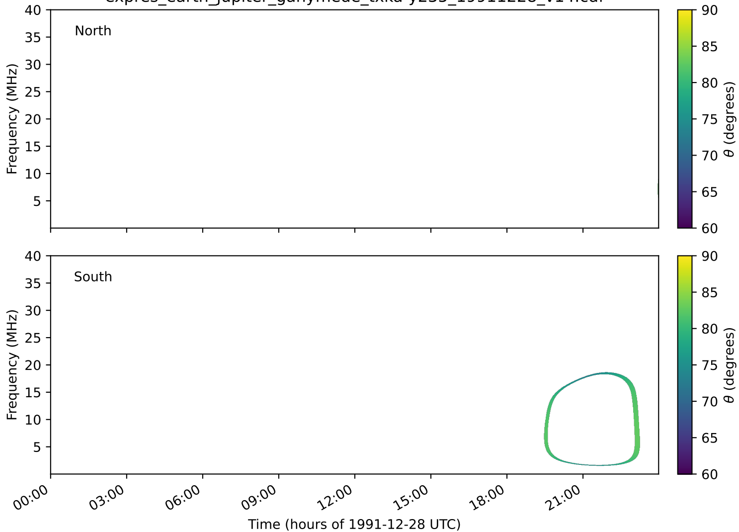
expres_earth_jupiter_ganymede_txka-y235_19911228_v14.cdf
