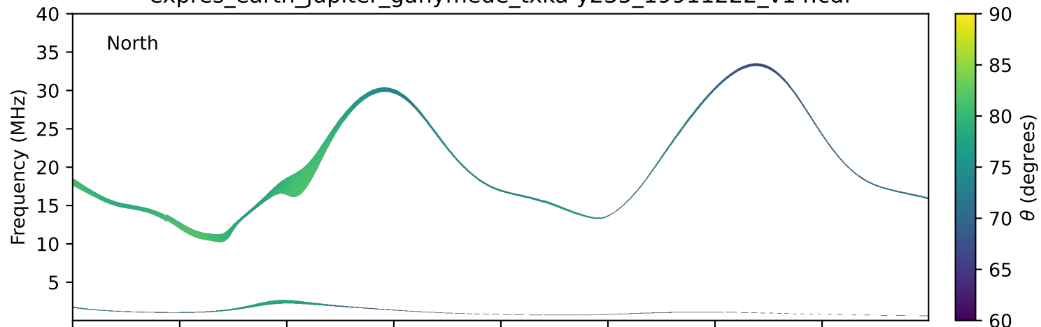
expres_earth_jupiter_ganymede_txka-y235_19911222_v14.cdf
