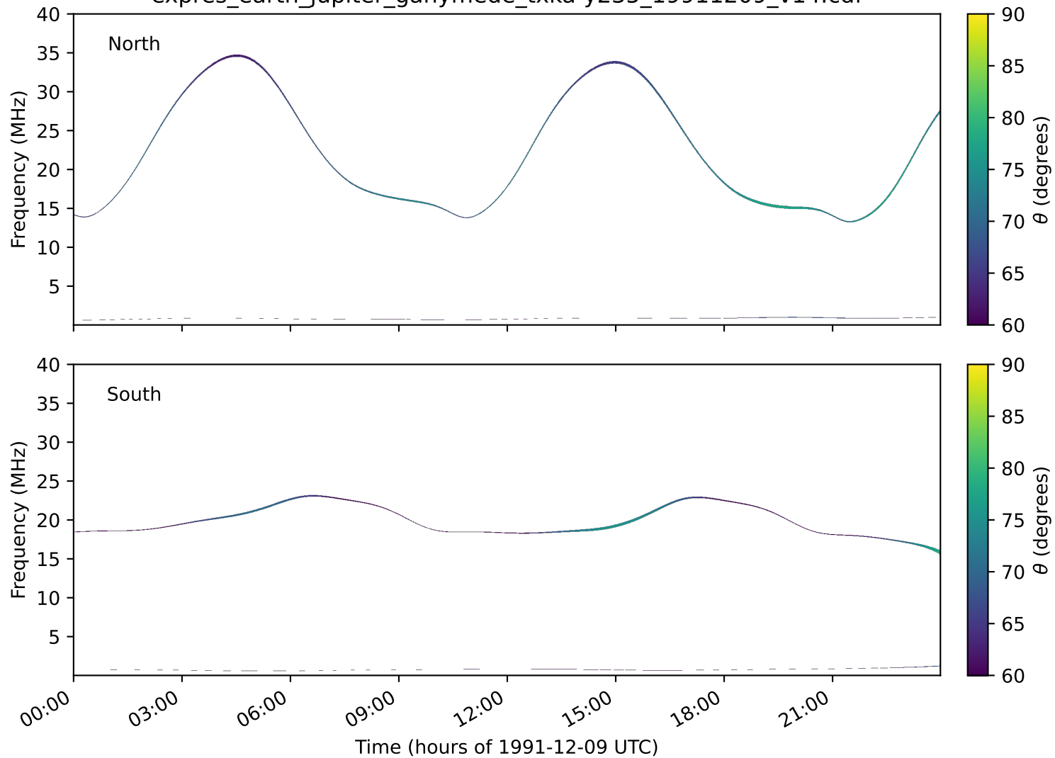
expres_earth_jupiter_ganymede_txka-y235_19911209_v14.cdf
