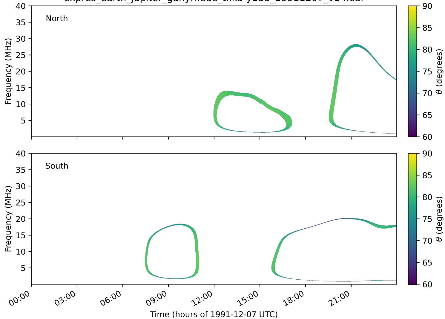
expres_earth_jupiter_ganymede_txka-y235_19911207_v14.cdf
