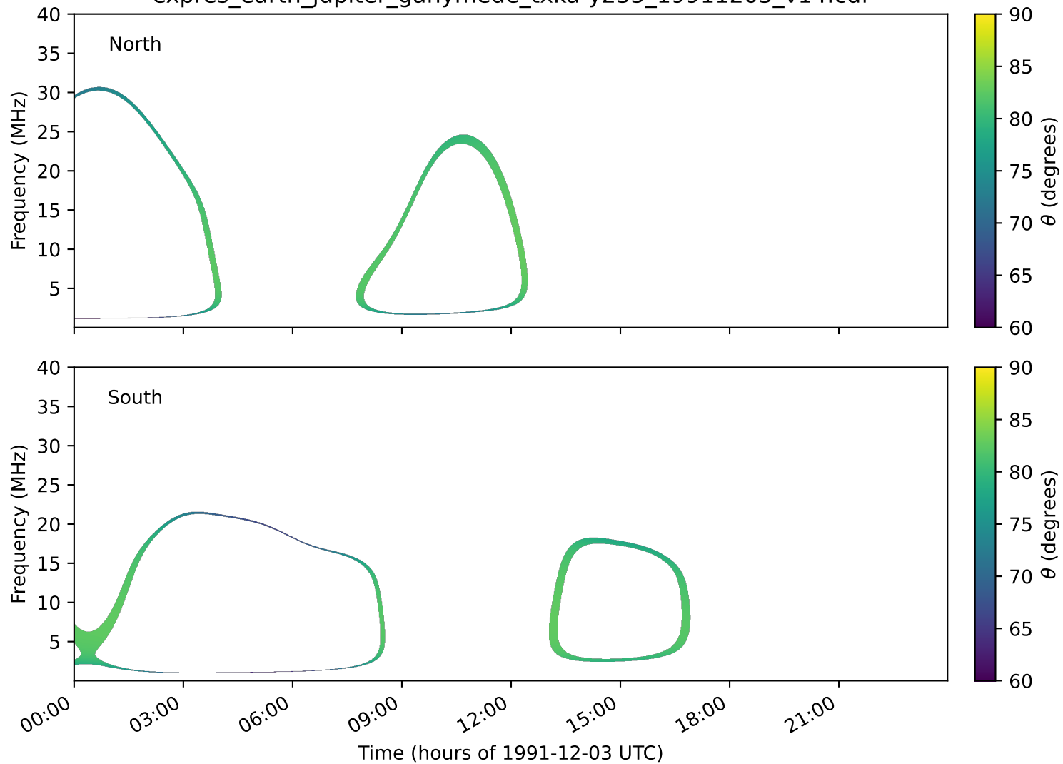
expres_earth_jupiter_ganymede_txka-y235_19911203_v14.cdf
