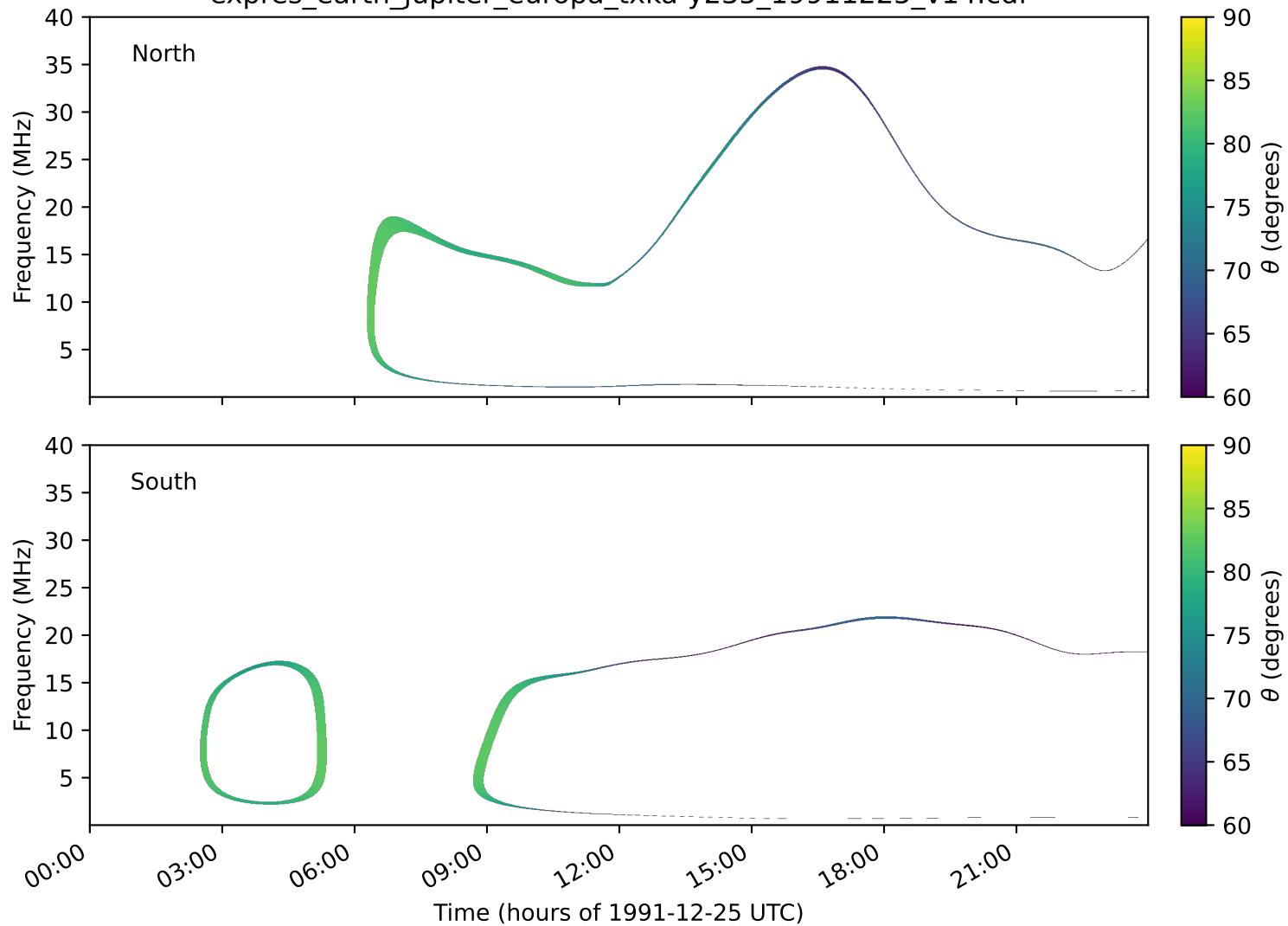
expres_earth_jupiter_europa_txka-y235_19911225_v14.cdf
