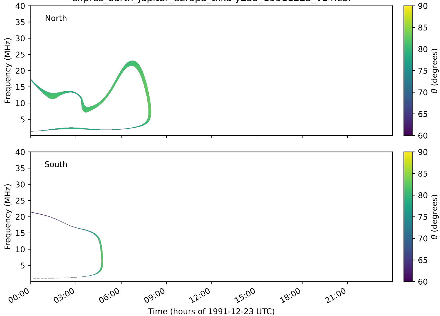
expres_earth_jupiter_europa_txka-y235_19911223_v14.cdf
