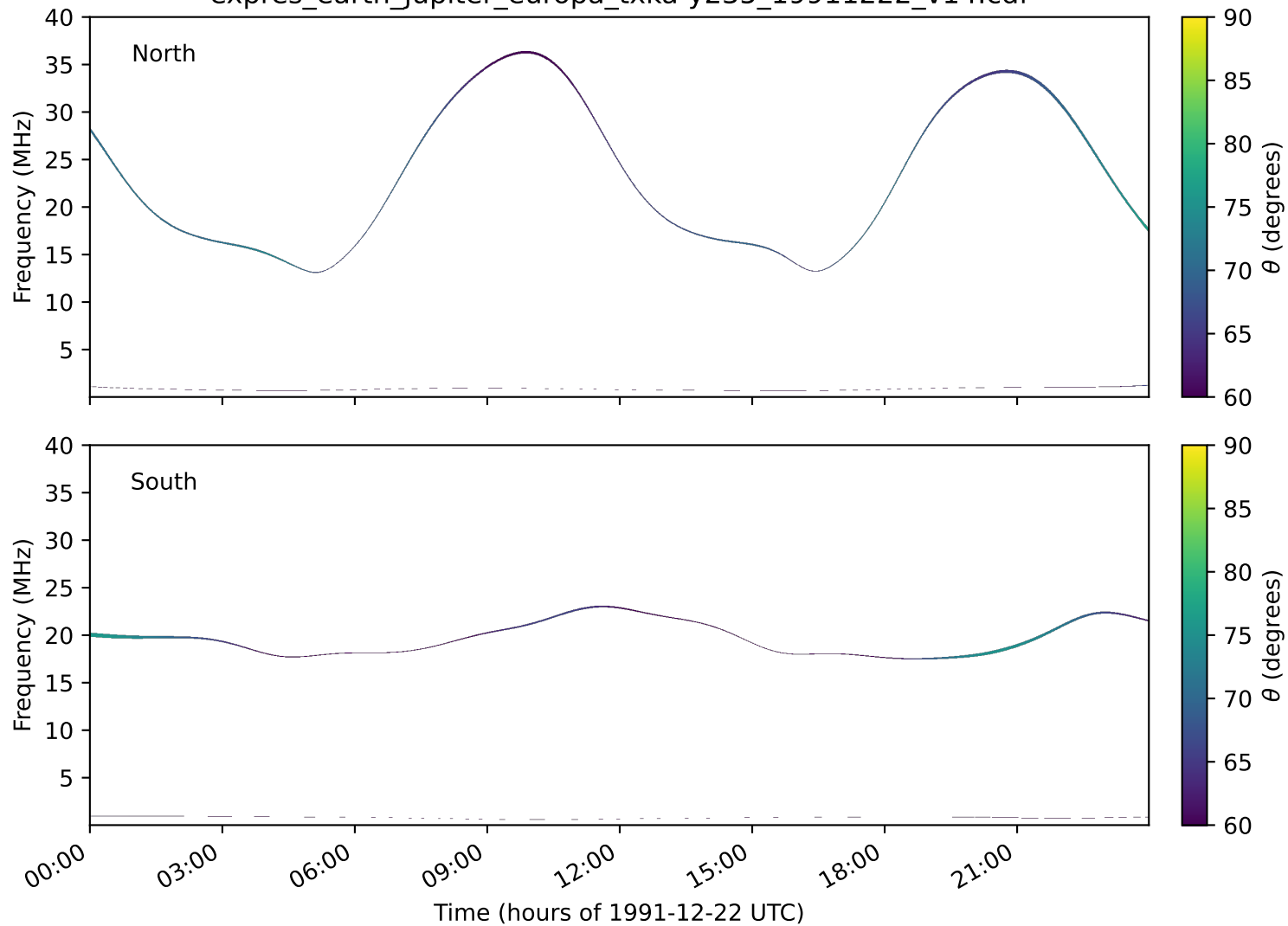
expres_earth_jupiter_europa_txka-y235_19911222_v14.cdf
