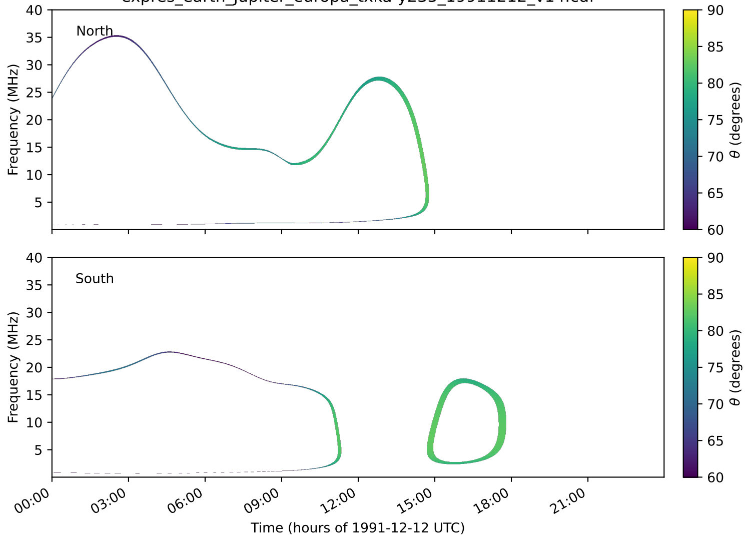
expres_earth_jupiter_europa_txka-y235_19911212_v14.cdf
