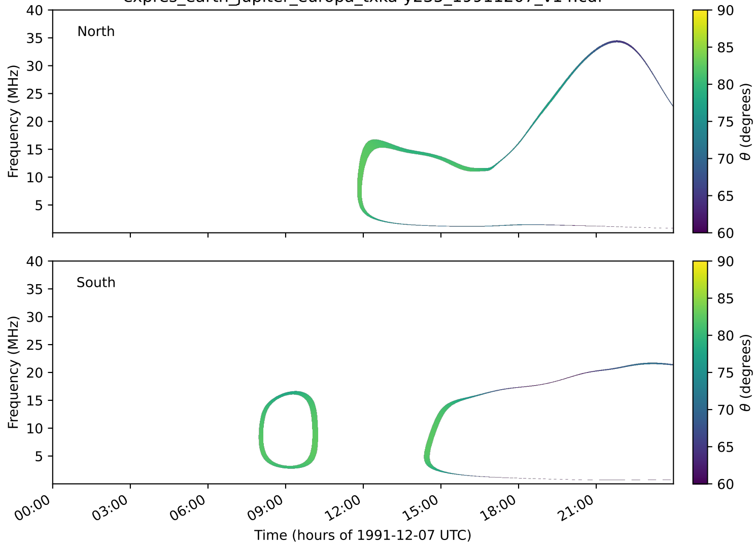
expres_earth_jupiter_europa_txka-y235_19911207_v14.cdf
