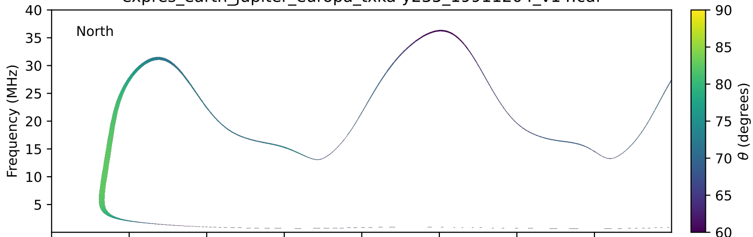
expres_earth_jupiter_europa_txka-y235_19911204_v14.cdf
