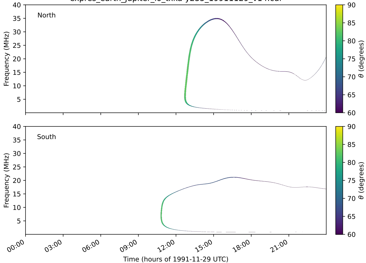
expres_earth_jupiter_io_txka-y235_19911129_v14.cdf
