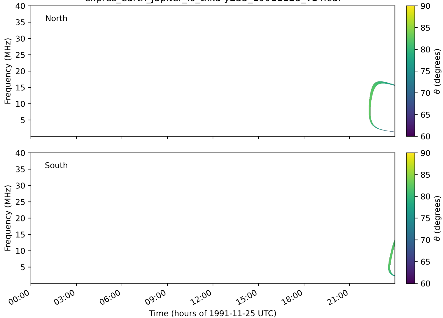
expres_earth_jupiter_io_txka-y235_19911125_v14.cdf
