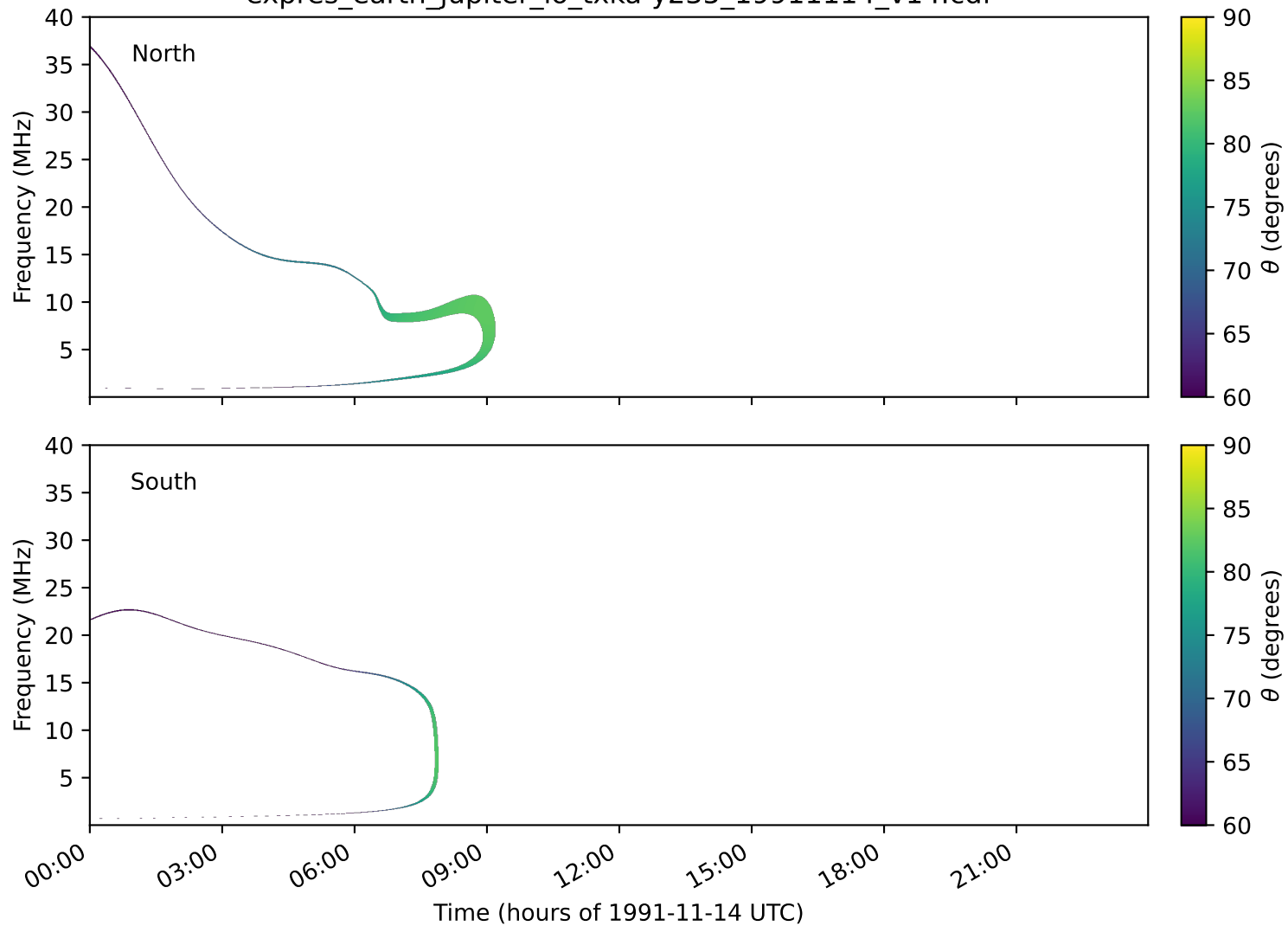
expres_earth_jupiter_io_txka-y235_19911114_v14.cdf
