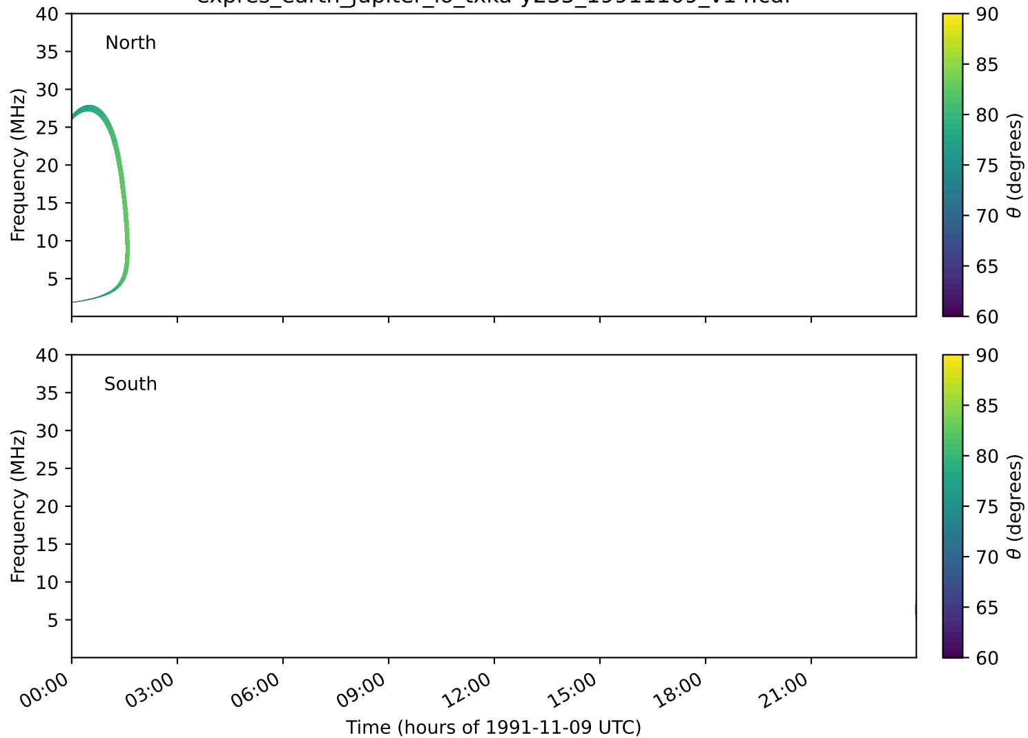
expres_earth_jupiter_io_txka-y235_19911109_v14.cdf
