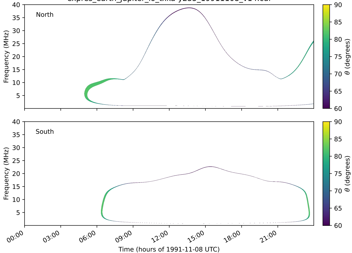
expres_earth_jupiter_io_txka-y235_19911108_v14.cdf
