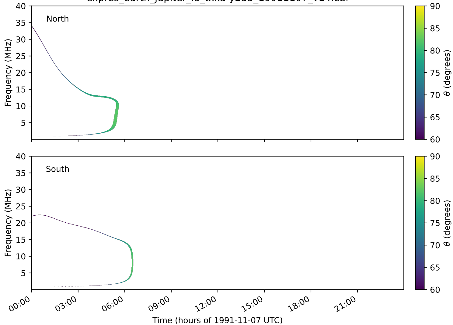
expres_earth_jupiter_io_txka-y235_19911107_v14.cdf
