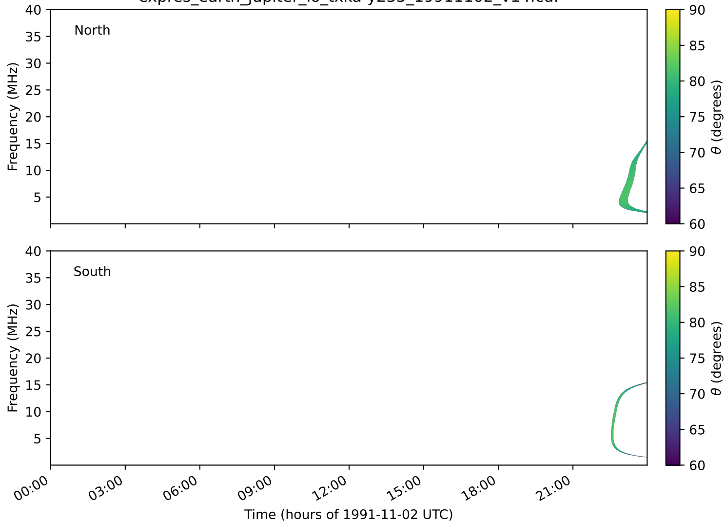
expres_earth_jupiter_io_txka-y235_19911102_v14.cdf
