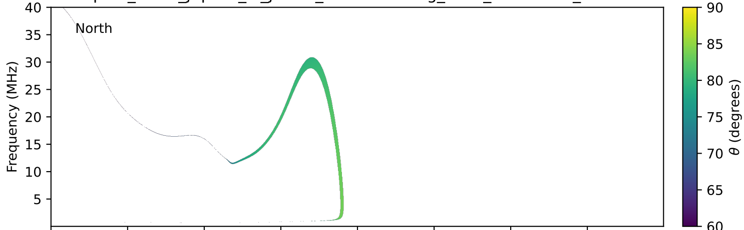
expres_earth_jupiter_io_jrm33_lossc-wid1deg_3kev_19911121_v11.cdf
