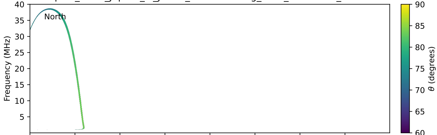
expres_earth_jupiter_io_jrm33_lossc-wid1deg_3kev_19911116_v11.cdf
