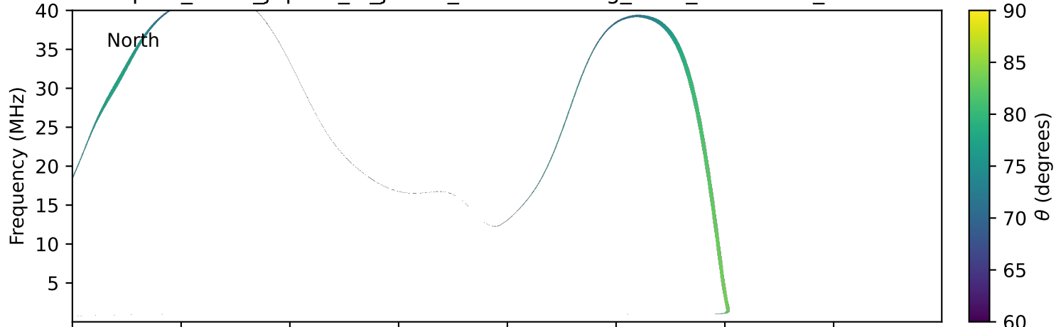
expres_earth_jupiter_io_jrm33_lossc-wid1deg_3kev_19911103_v11.cdf
