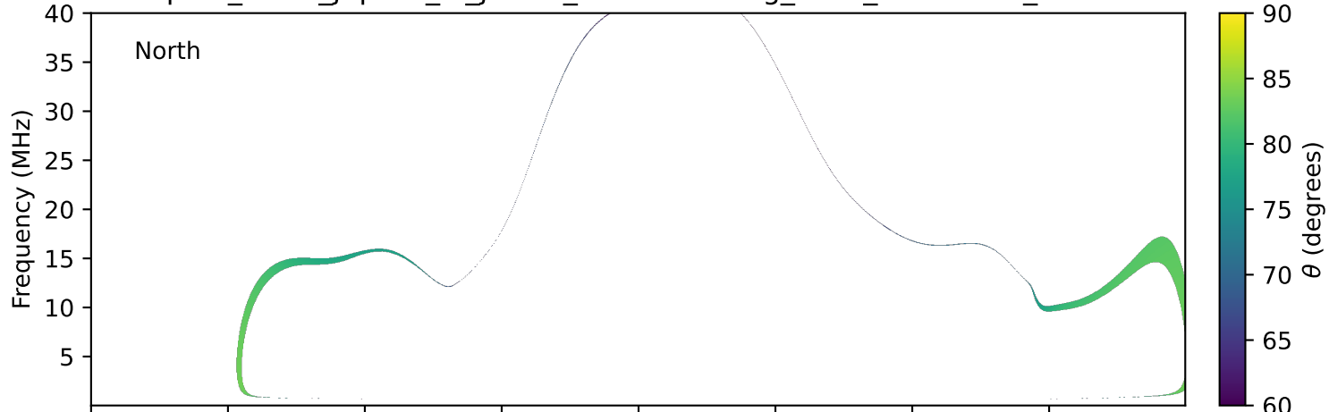
expres_earth_jupiter_io_jrm33_lossc-wid1deg_3kev_19911101_v11.cdf
