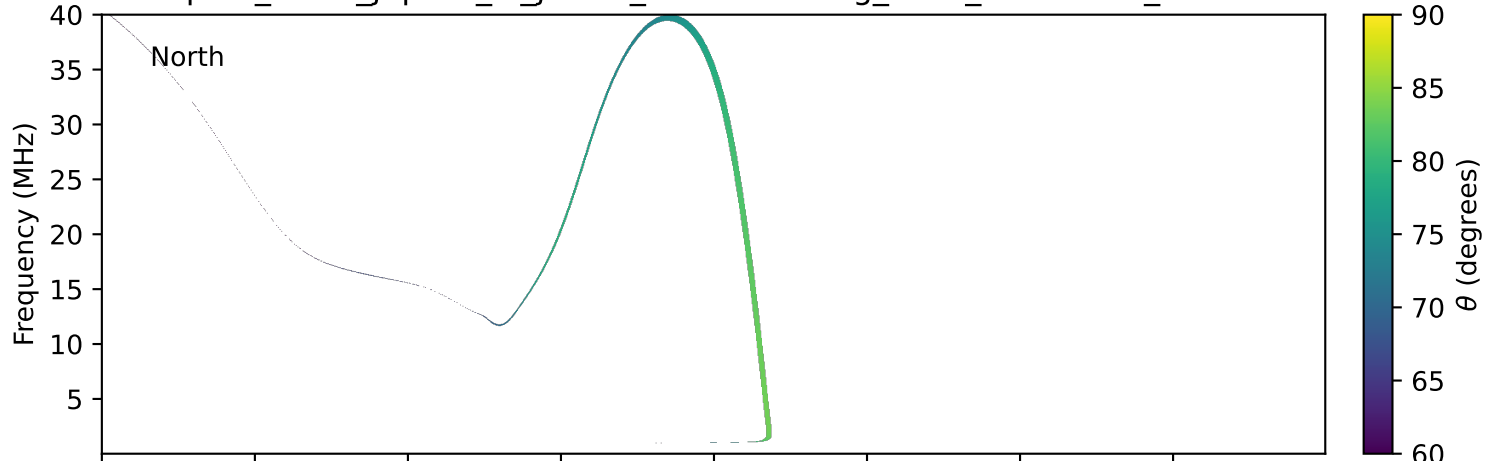
expres_earth_jupiter_io_jrm09_lossc-wid1deg_3kev_19911128_v11.cdf
