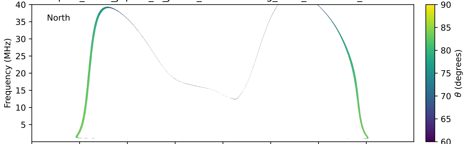
expres_earth_jupiter_io_jrm09_lossc-wid1deg_3kev_19911117_v11.cdf
