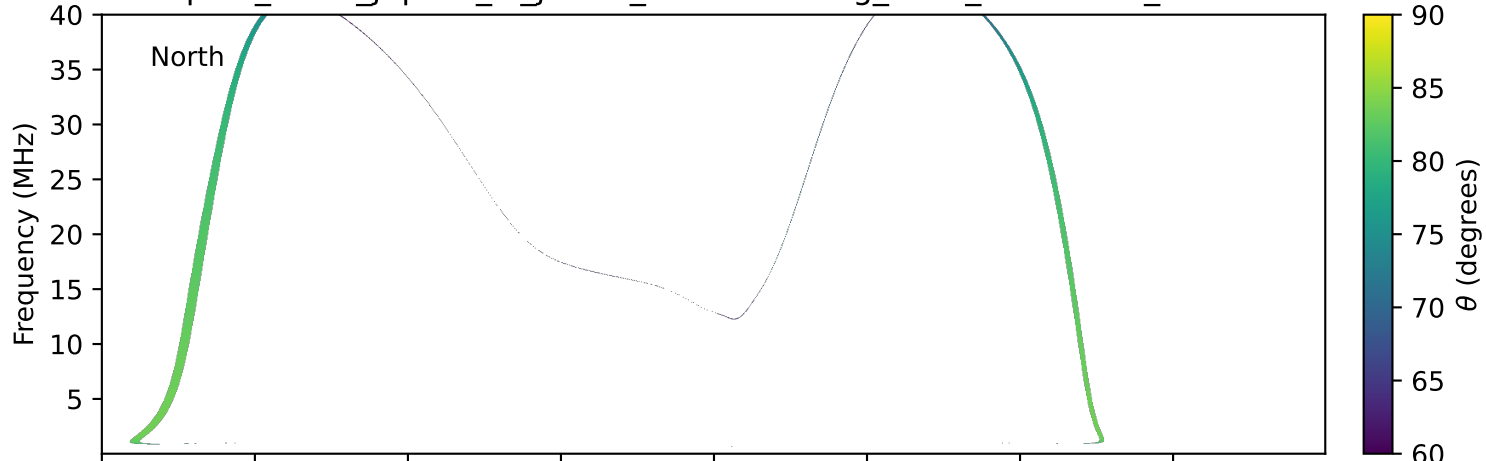
expres_earth_jupiter_io_jrm09_lossc-wid1deg_3kev_19911110_v11.cdf
