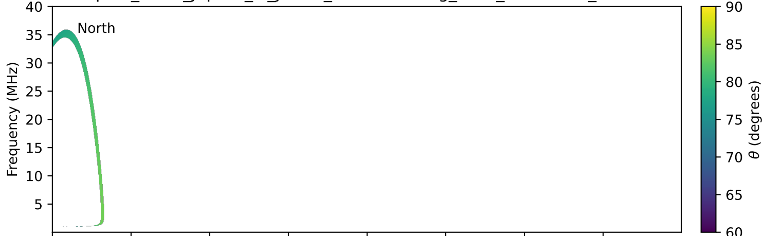
expres_earth_jupiter_io_jrm09_lossc-wid1deg_3kev_19911109_v11.cdf
