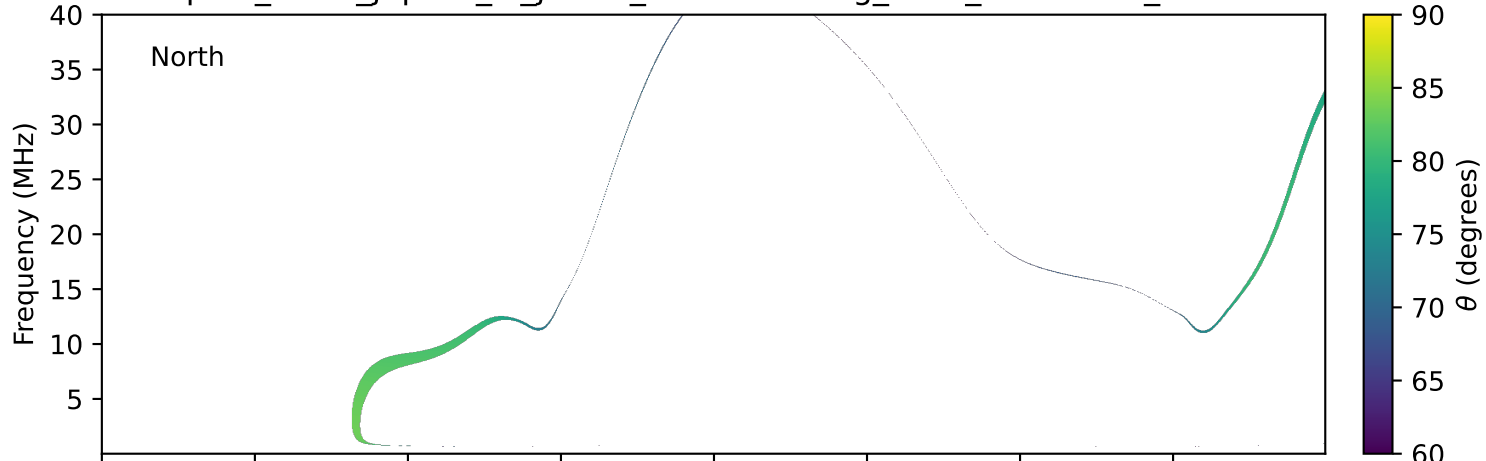
expres_earth_jupiter_io_jrm09_lossc-wid1deg_3kev_19911108_v11.cdf
