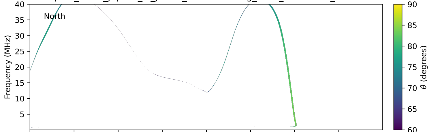
expres_earth_jupiter_io_jrm09_lossc-wid1deg_3kev_19911103_v11.cdf
