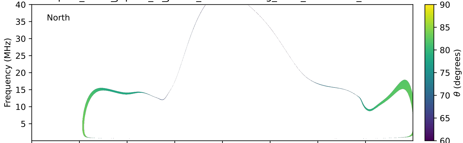
expres_earth_jupiter_io_jrm09_lossc-wid1deg_3kev_19911101_v11.cdf
