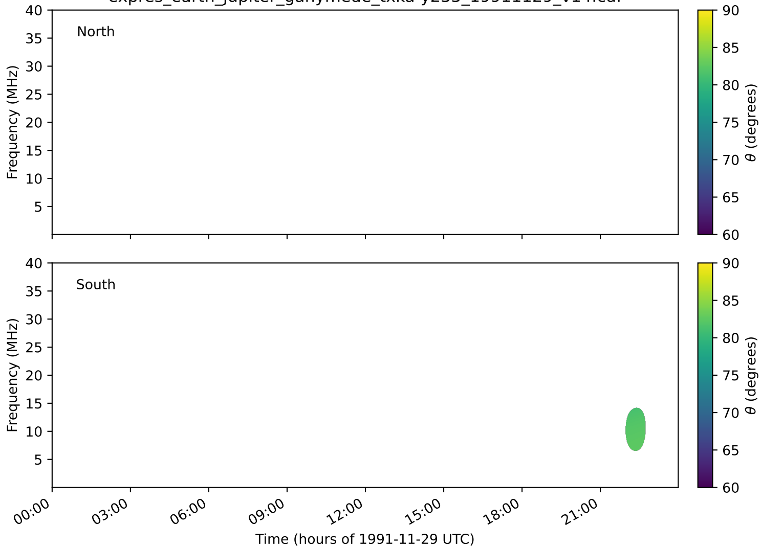
expres_earth_jupiter_ganymede_txka-y235_19911129_v14.cdf
