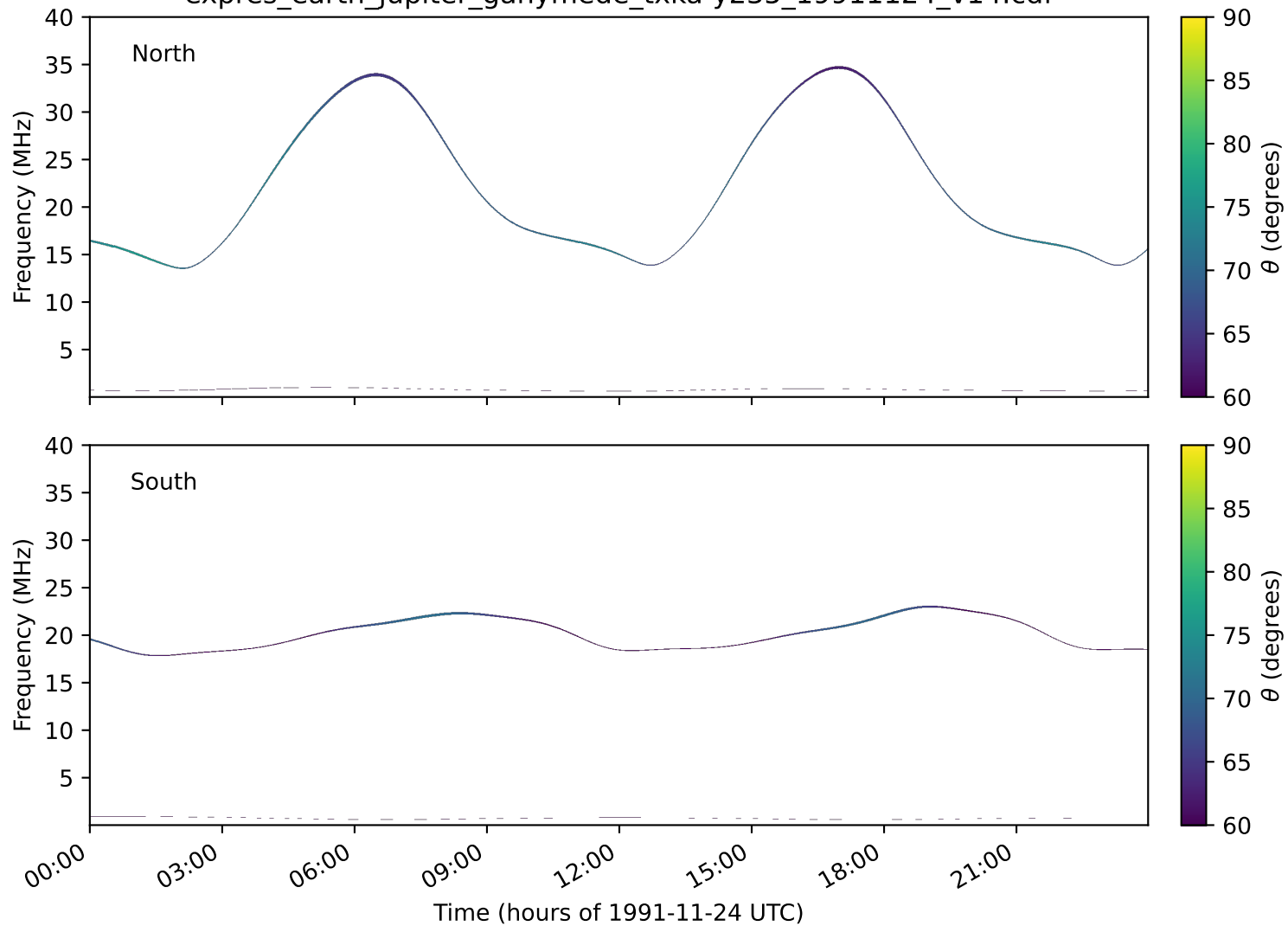
expres_earth_jupiter_ganymede_txka-y235_19911124_v14.cdf
