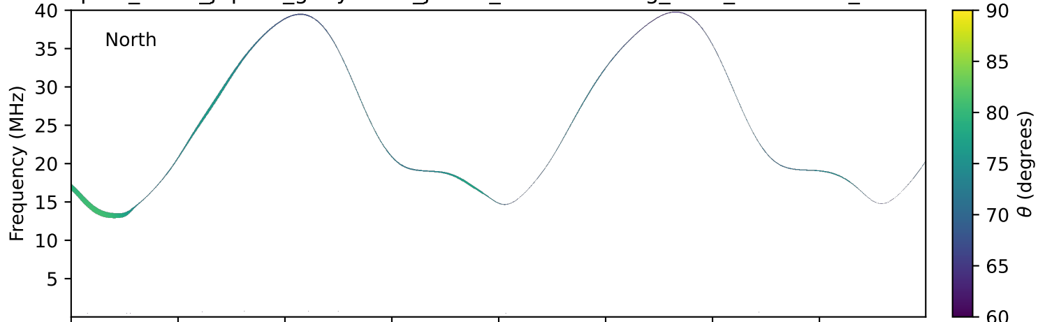
expres_earth_jupiter_ganymede_jrm33_lossc-wid1deg_3kev_19911124_v11.cdf
