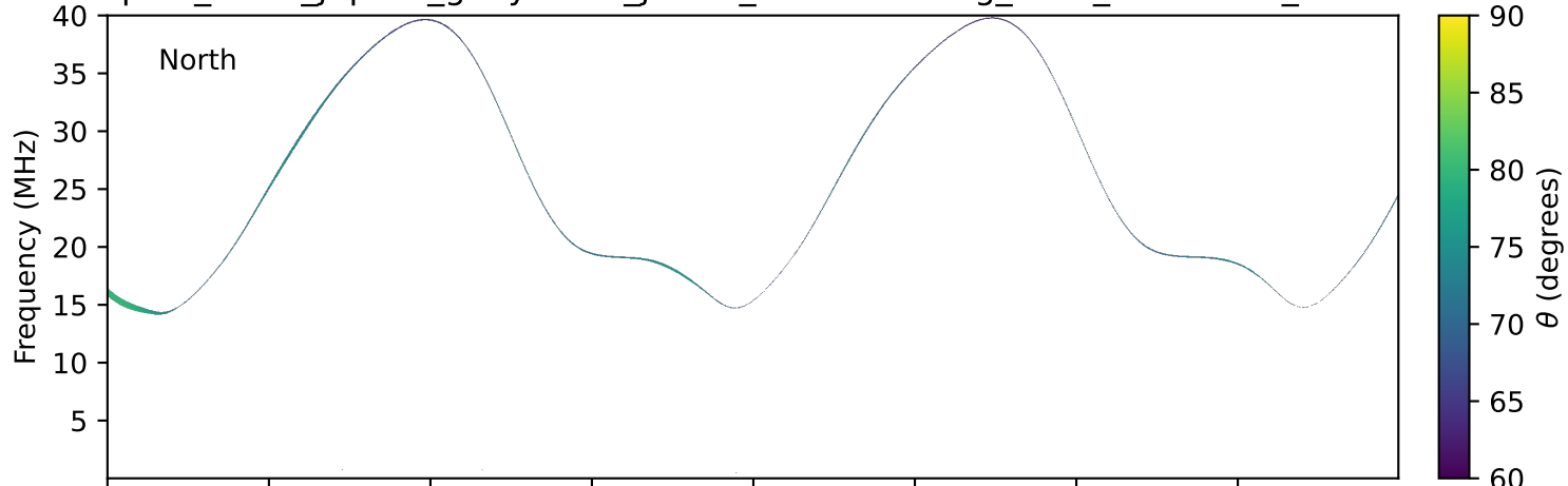
expres_earth_jupiter_ganymede_jrm33_lossc-wid1deg_3kev_19911117_v11.cdf
