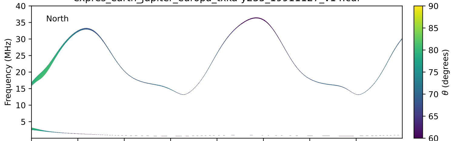
expres_earth_jupiter_europa_txka-y235_19911127_v14.cdf
