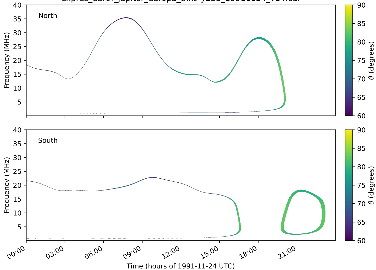
expres_earth_jupiter_europa_txka-y235_19911124_v14.cdf
